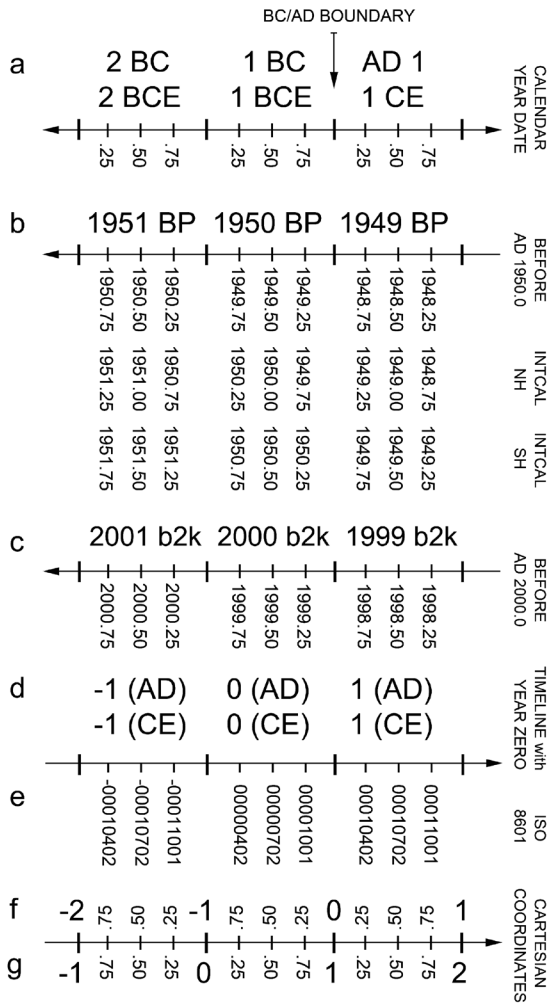
Fig. 1 - A comparison of timelines and notations. a) Calendric dates as ordinal numbers, each integral number designating an entire calendar year, with associated decimally expressed sub-annual dates. b) Before Present (BP) age as integral numbers relative to AD 1950 and with associated decimally expressed sub-annual ages, where 0.0 cal BP equals either AD 1950.0 (Holden et al. , 2011), AD 1950.5 (IntCal Northern Hemisphere (NH)), or AD 1951.0 (Intcal Southern Hemisphere (SH)). c) Before AD 2000 (b2k) ages as integral numbers and with associated decimally expressed sub-annual ages relative to AD 2000.0. d) Calendar years as negative and positive numbers relative to AD (and CE) timescale, following Schulman (1956). e) Calendar dates using the ISO 8601 standard. f) Dates plotted as floating-point numbers on Cartesian coordinates where the zero-point is placed at 1BC/AD1 (that is the BC/AD boundary). g) Same as f but the zero-point is placed at 2BC/1BC. The BC/AD boundary is marked with a downward arrow. BP ages refer to cal BP timeline. / Confronto tra cronologie e notazioni. a) Date calendariali come numeri ordinali, in cui ciascun numero intero designa un intero anno del calendario, con associate date sub-annuali espresse in forma decimale. b) Età Before Present (BP) come numeri interi riferiti al 1950 d.C., con età sub-annuali espresse in formato decimale; 0,0 cal BP corrisponde infatti a 1950,0 d.C. (Holden et al. , 2011), 1950,5 d.C. (IntCal Northern Hemisphere (NH)) oppure 1951,0 d.C. (IntCal Southern Hemisphere (SH)). c) Età Before AD 2000 (b2k) come numeri interi, con età sub-annuali espresse in formato decimale rispetto al 2000,0 d.C. d) Anni del calendario espressi come numeri negativi e positivi rispetto alla scala temporale d.C. (e C.E.), secondo Schulman (1956). e) Date calendariali secondo lo standard ISO 8601. f) Date rappresentate come numeri in virgola mobile su coordinate cartesiane, con il punto zero posto a 1 a.C./1 d.C. (ossia il limite a.C./d.C.). g) Come in f), ma con il punto zero posto a 2 a.C./1 a.C. Il limite a.C./d.C. è indicato con una freccia rivolta verso il basso. Le età BP si riferiscono alla cronologia cal BP.
